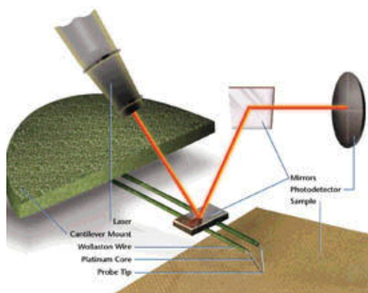
FIGURE 1 SCHEME OF AFM ARRANGEMENT [6]
