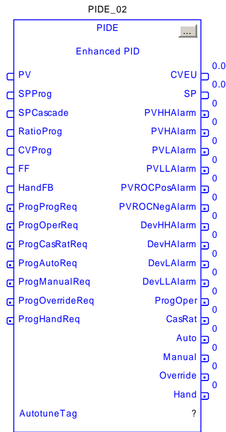
FIGURE 1 PIDE FUNCTION BLOCK
