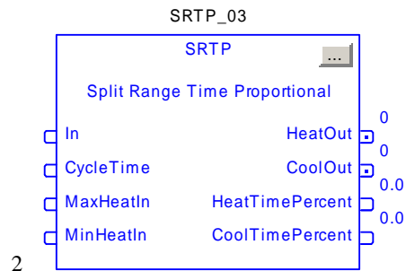
FIGURE 2 SPLIT RANGE TIME PROPORTIONAL
