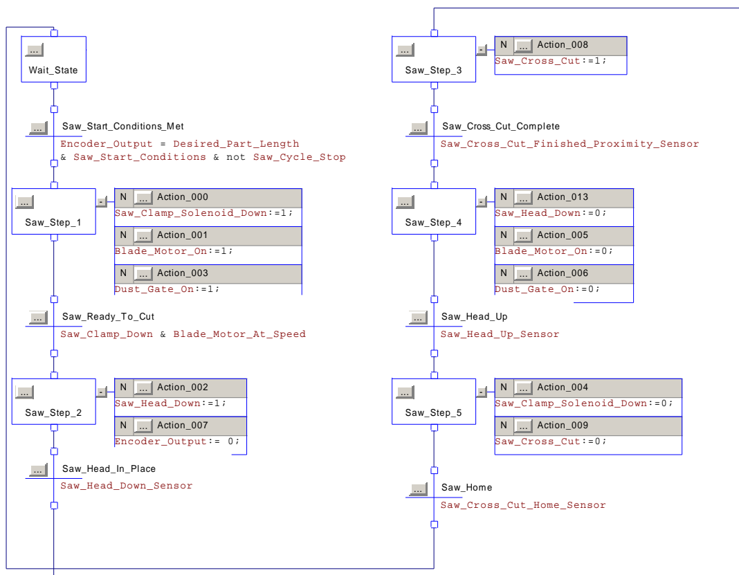
FIGURE 6 NEW SAW CODE IN SEQUENTIAL FUNCTION CHART AS PROGRAMMED IN RSLOGIX5000
