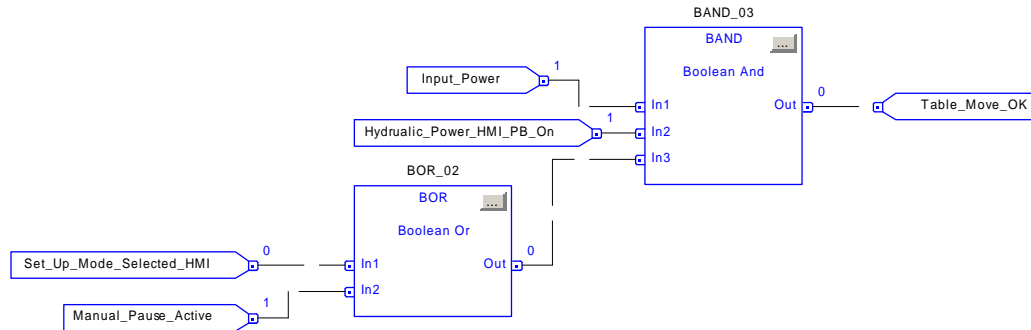
FIGURE 8 NEW DIE SET-UP CODE IN FUNCTIONAL BLOCK DIAGRAM AS PROGRAMMED IN RSLOGIX5000
