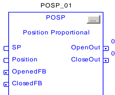
FIGURE 3 POSITION PROPORTIONAL
